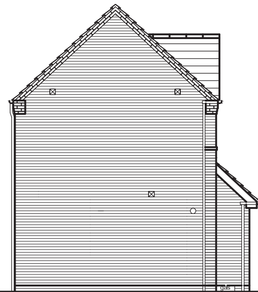
REAR ELEVATION
